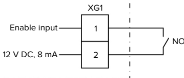
Fig. 13: Schematic circuit diagram: Connection of an external switching contact
